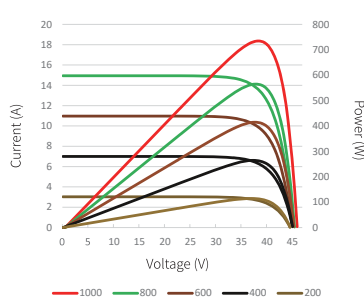
Current-Voltage & Power-Voltage Curves (720W)
